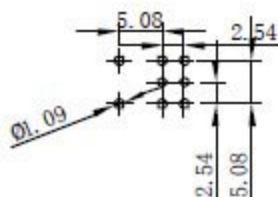
P.C.B MOUNTING DIMENSION
