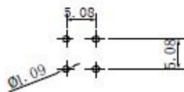
P.C.B MOUNTING DIMENSION
